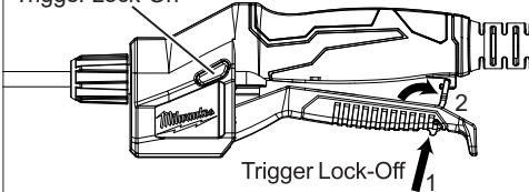
Trigger Lock-On
